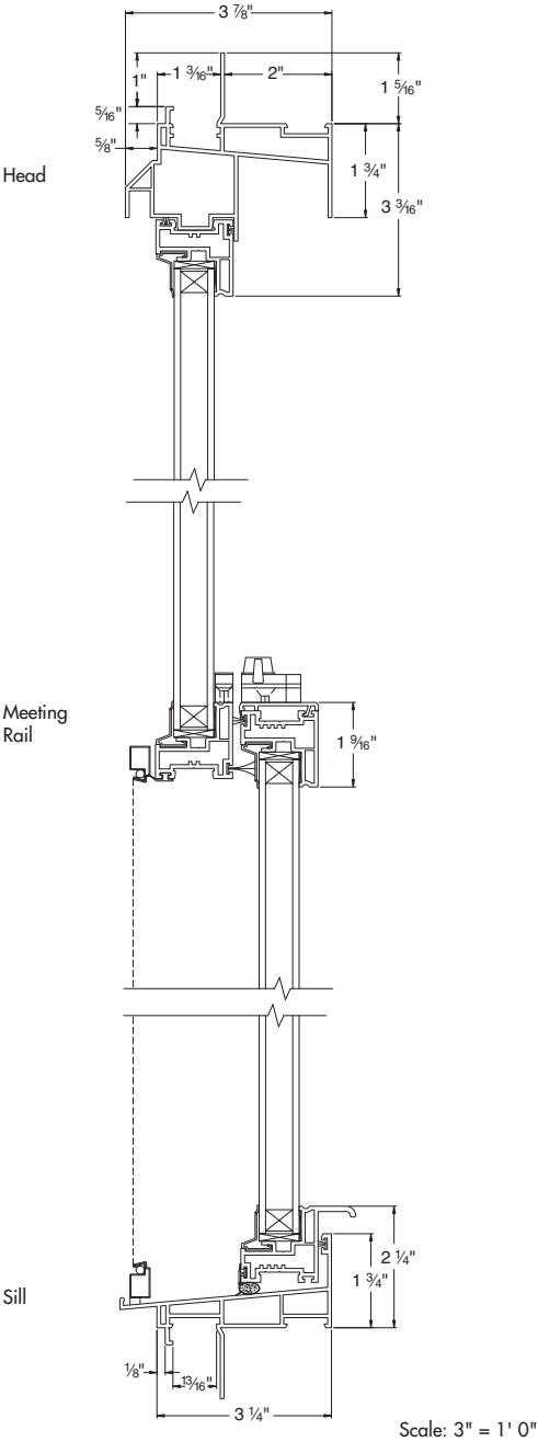
Single-Hung – Vertical Detail
