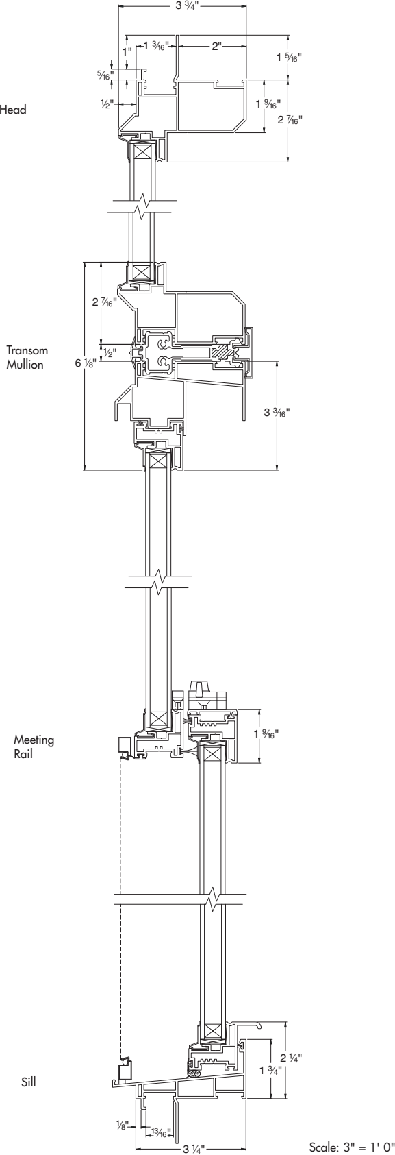
Single-Hung with Transom – Vertical Detail (Factory Mullion Shown)
