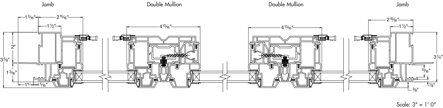
Casement/Fixed/Casement – Horizontal Detail
