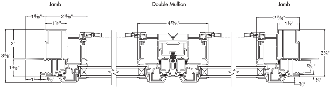
Twin Casement – Horizontal Detail
