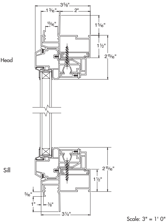
Casement Picture (Fixed) – Vertical Detail
