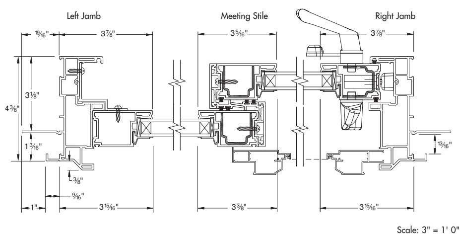
Standard Patio Door – Horizontal Detail
