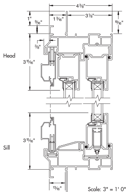
Standard Patio Door – Vertical Detail
