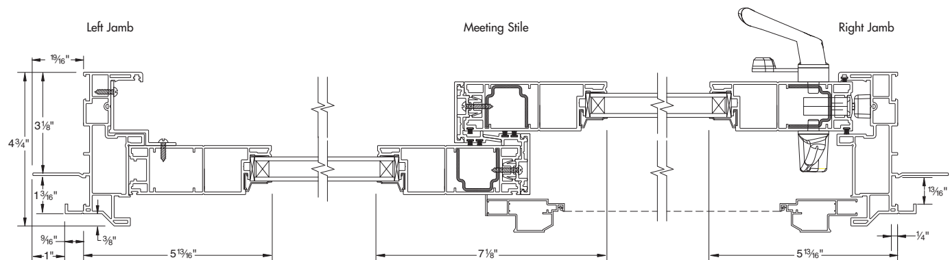
French Patio Door – Horizontal Detail
